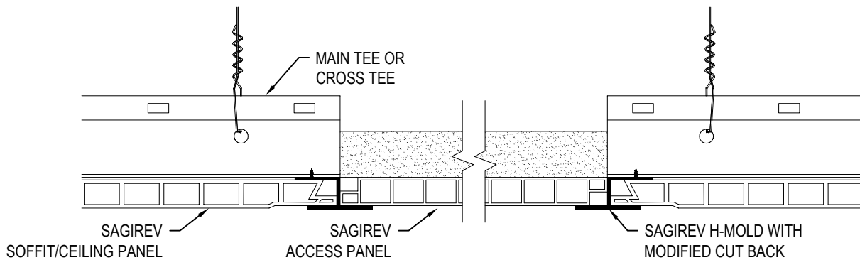
SECTION VIEW
