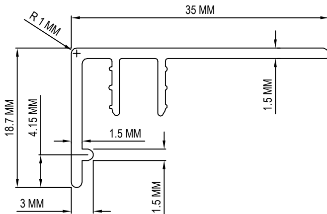
TERMINATING J-MOLD PROFILE
