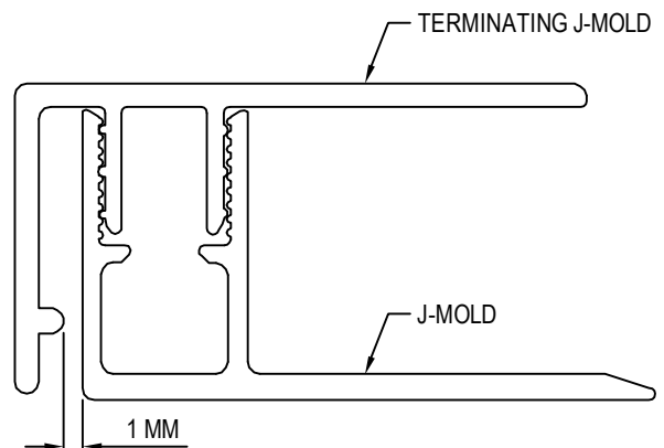
TERMINATING J-MOLD WITH J-MOLD PROFILE
