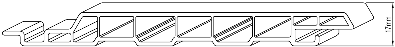
SAGIWALL PROFILE
