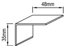
ALUMINUM CORNER 35mm X 48mm
