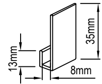
ALUM. STARTER STRIP
