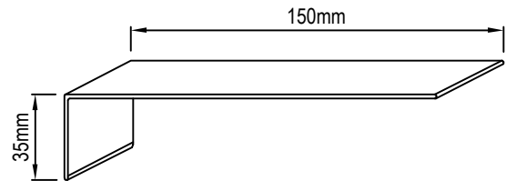
ALUMINUM CORNER 35mm X 150mm
