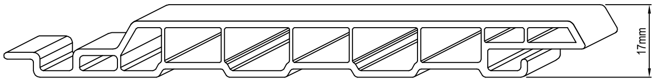
SAGIWALL PROFILE
