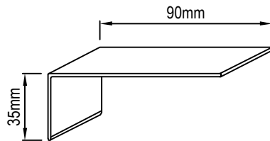
ALUMINUM CORNER 35mm X 90mm
